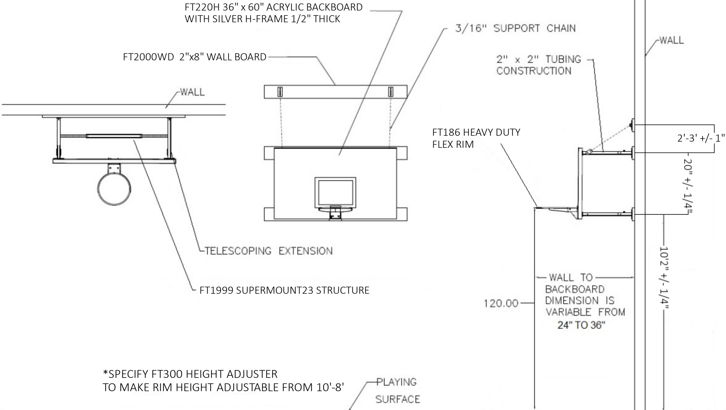
FRONT VIEW
