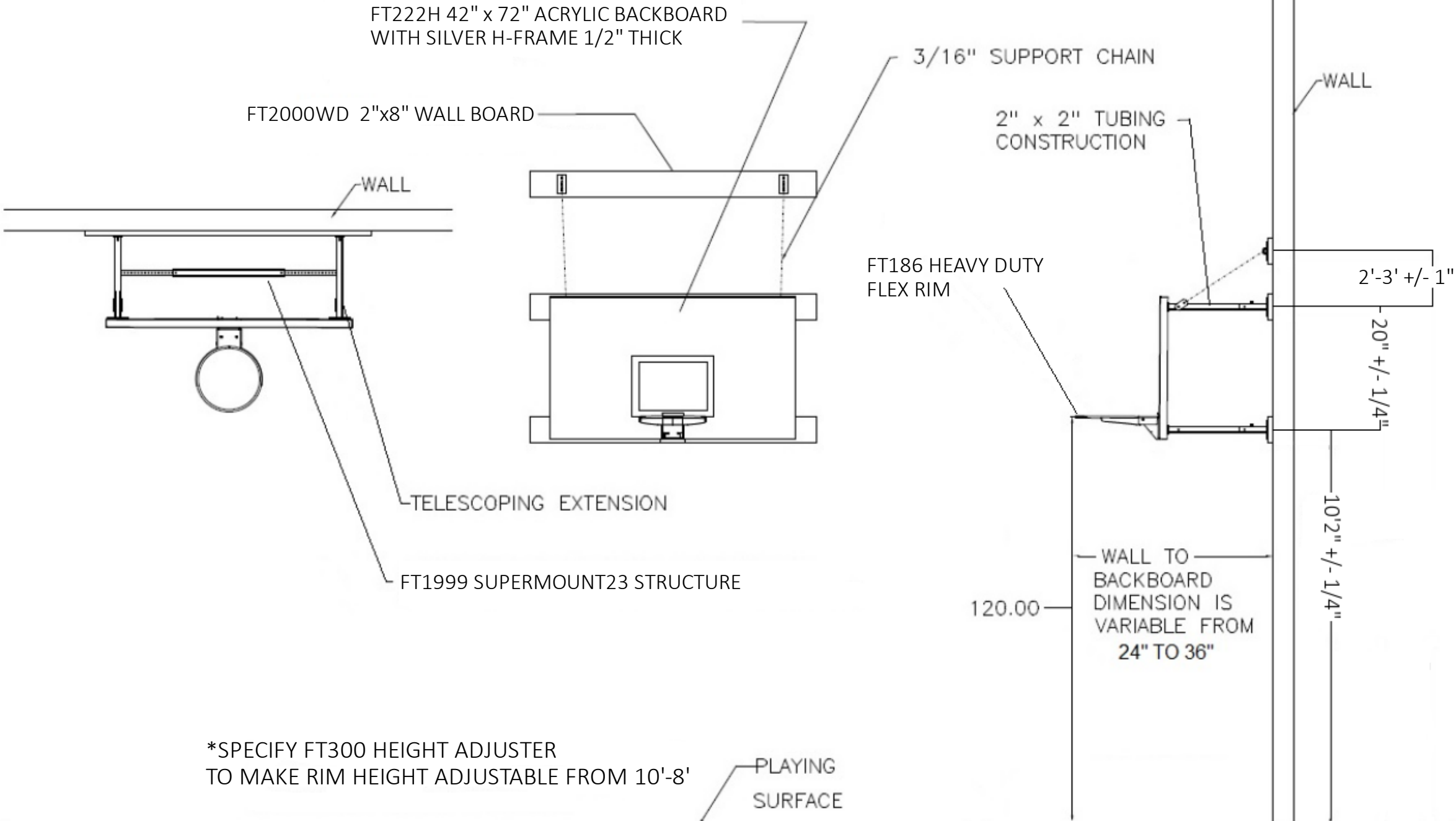
FRONT VIEW
