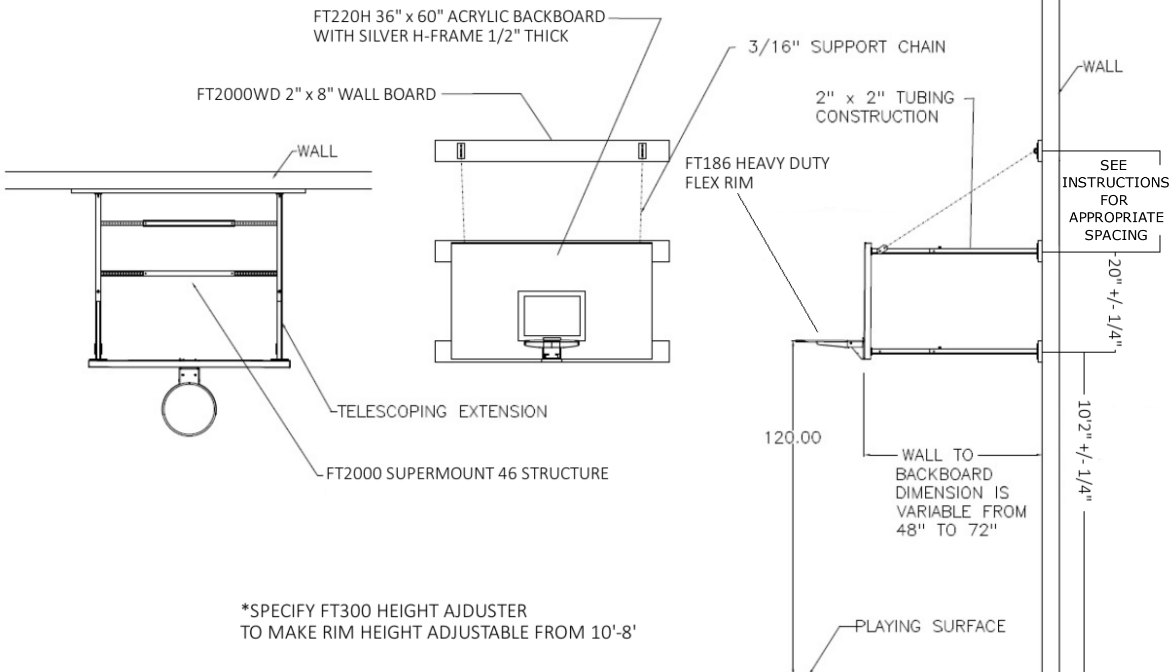
FRONT VIEW
