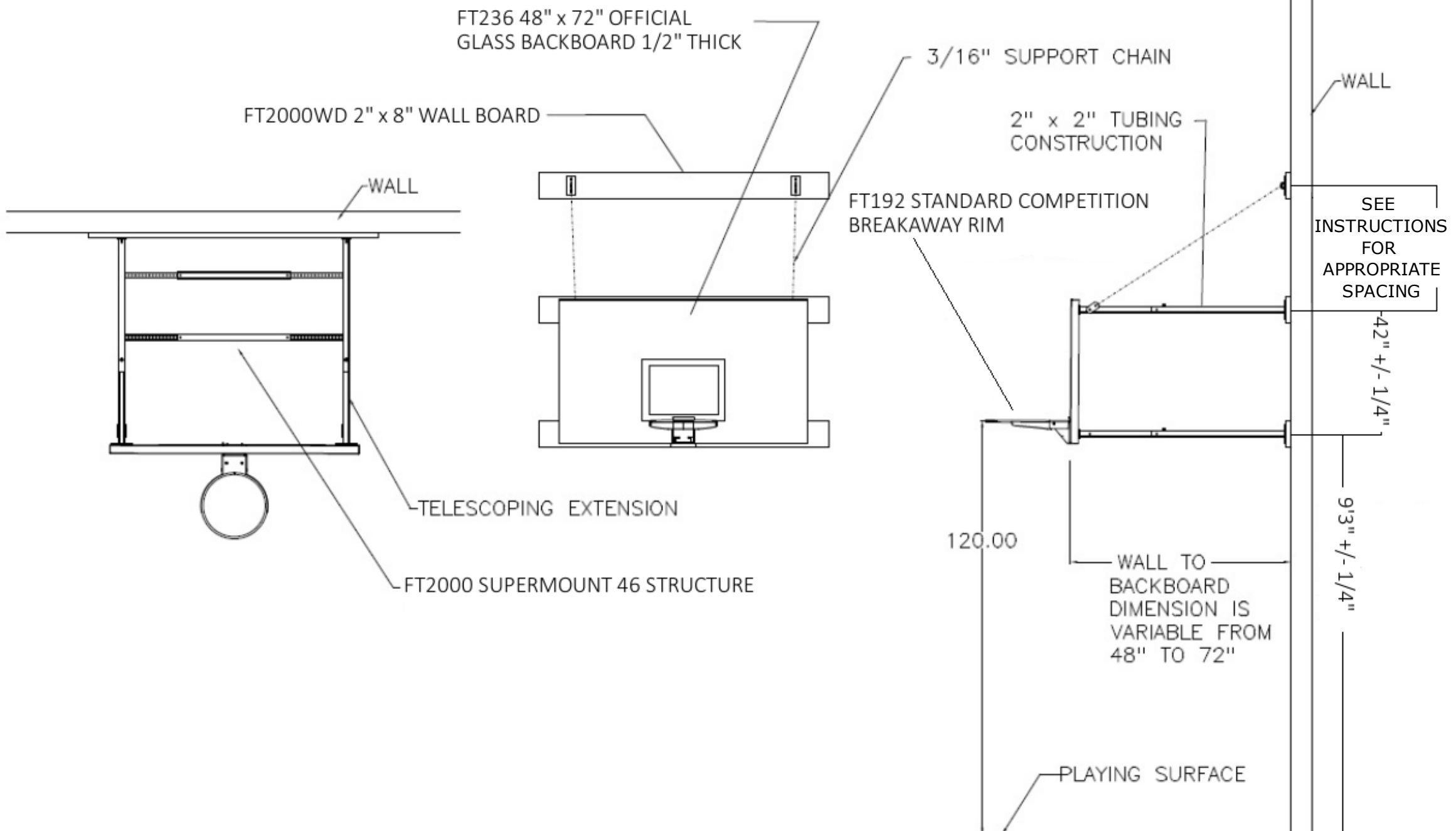
FRONT VIEW
