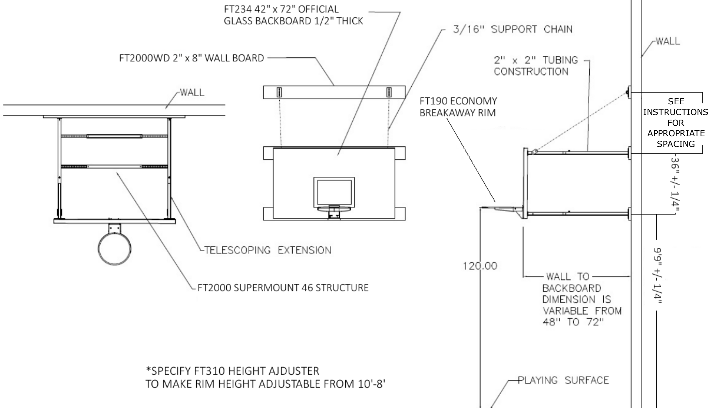
FRONT VIEW
