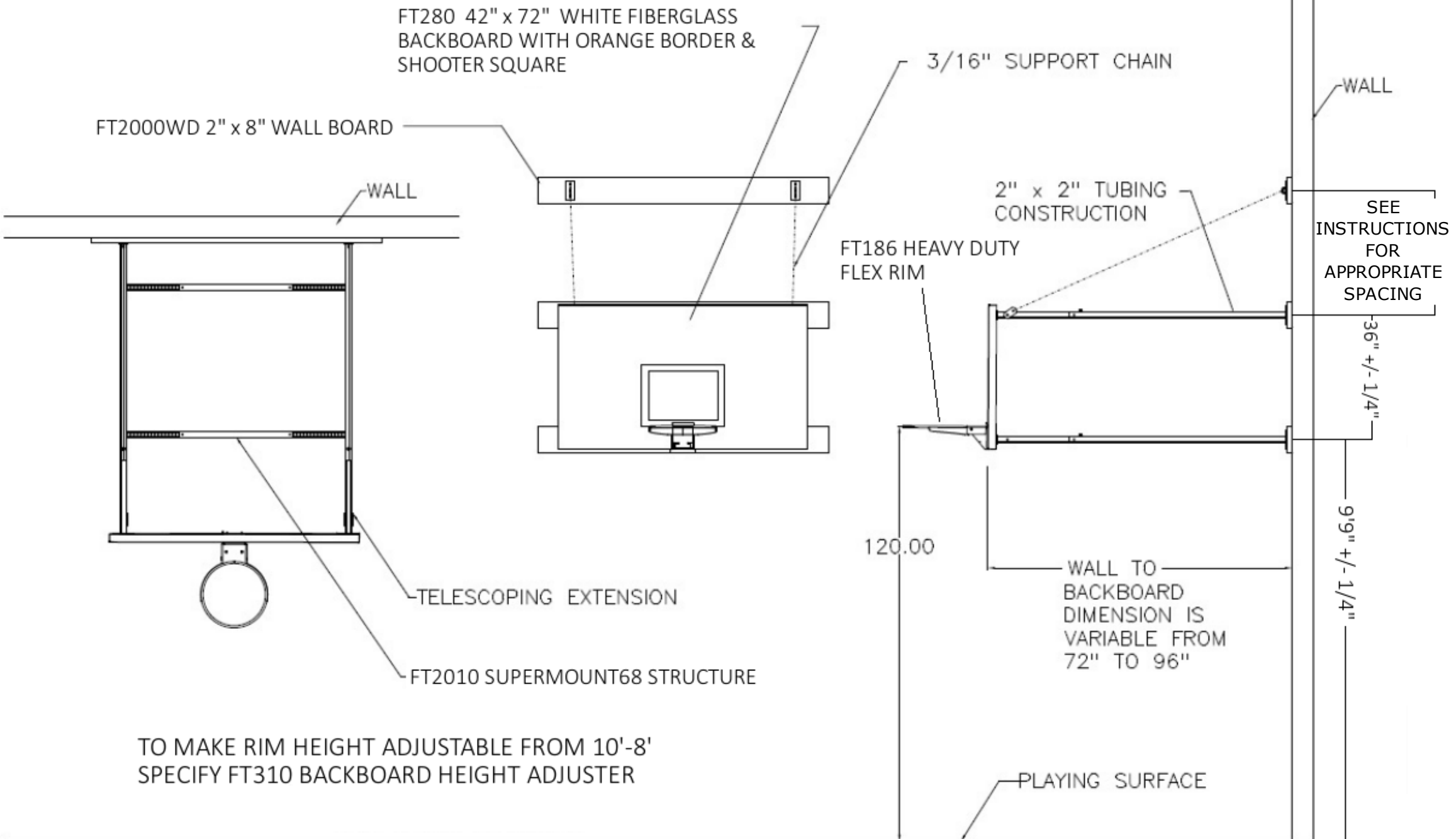
FRONT VIEW
