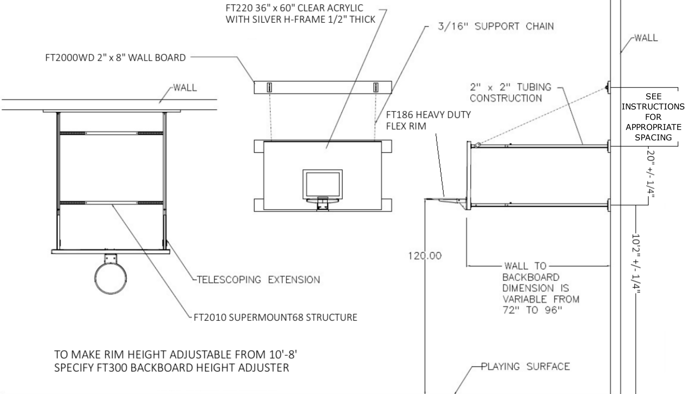
FRONT VIEW
